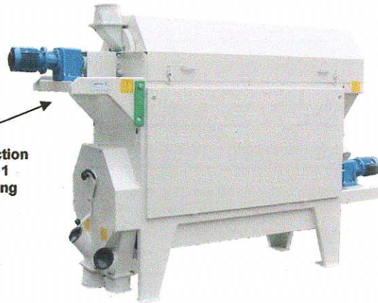
H-500 x 1500 up to 2 t/h H-500 x 1900 up to 3 t/h H-500 x 2500 up to 4 t/h
