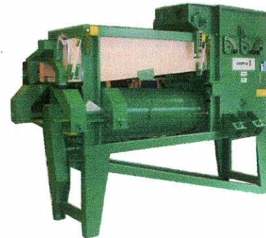
S-600 up to 2.0 t/h S-1250 up to 4.0 t/h
